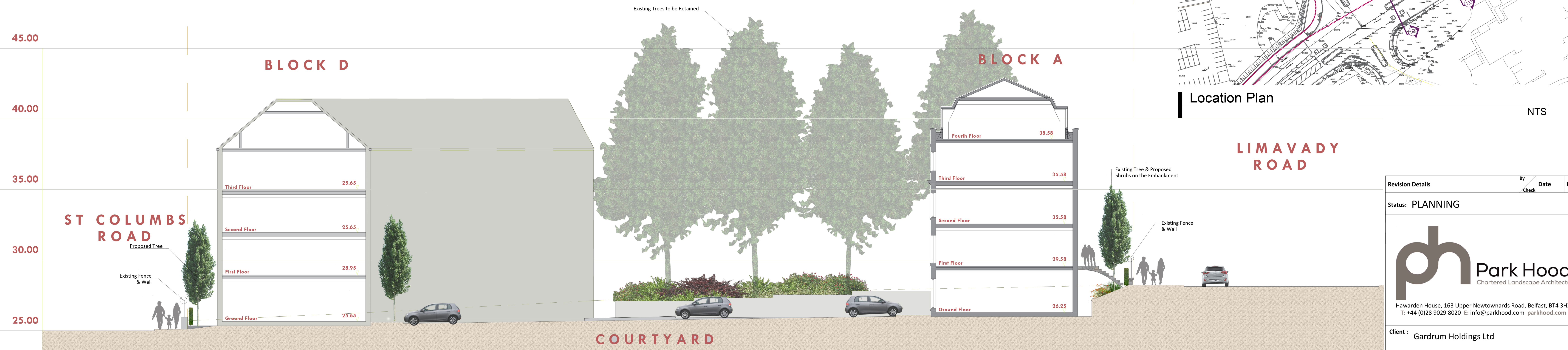
Landscape Section Section B-B
