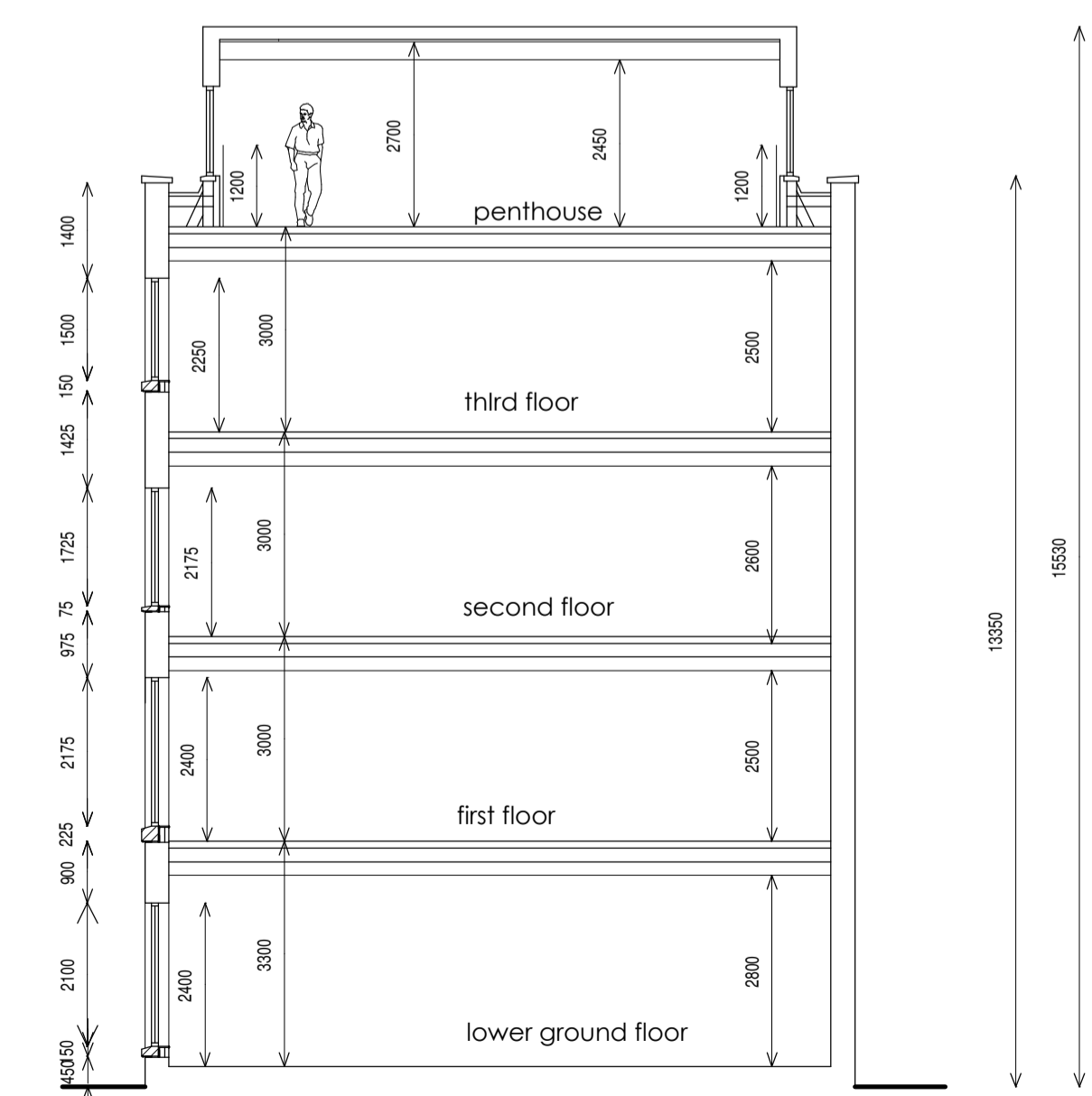
Section A-A (Thro block A)
