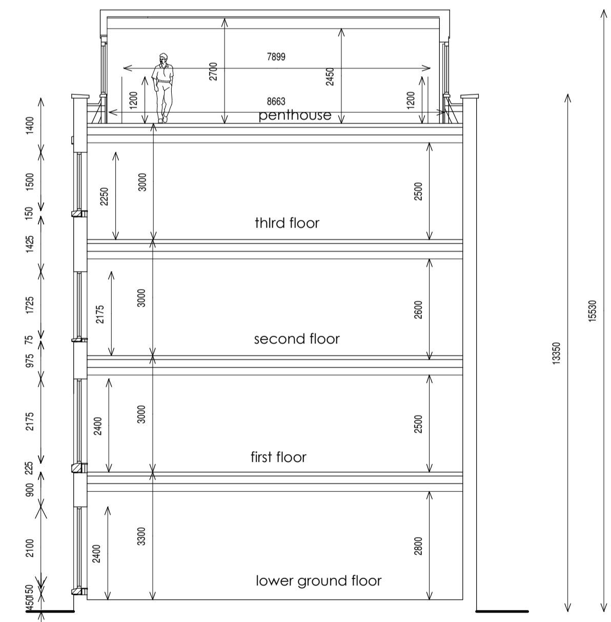
Section A-A (Thru block A)
