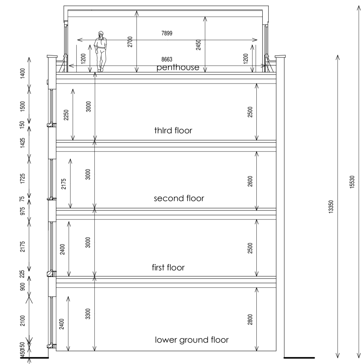
Section A-A (Through Block A)
